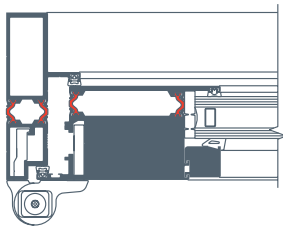
4" Frame Polyamide Thermal Break (shown in red)
