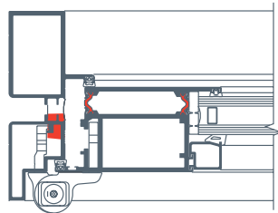
5" Frame Pour and Debridge Thermal Break (shown in red)
